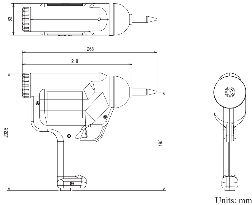
Fig. 8-1 Outline Drawing of Discharge Gun
