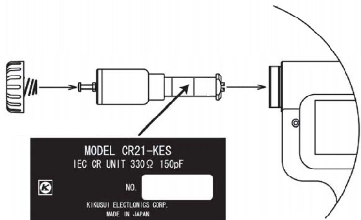
Fig. 2-2 Checking the CR Unit Constant Values
