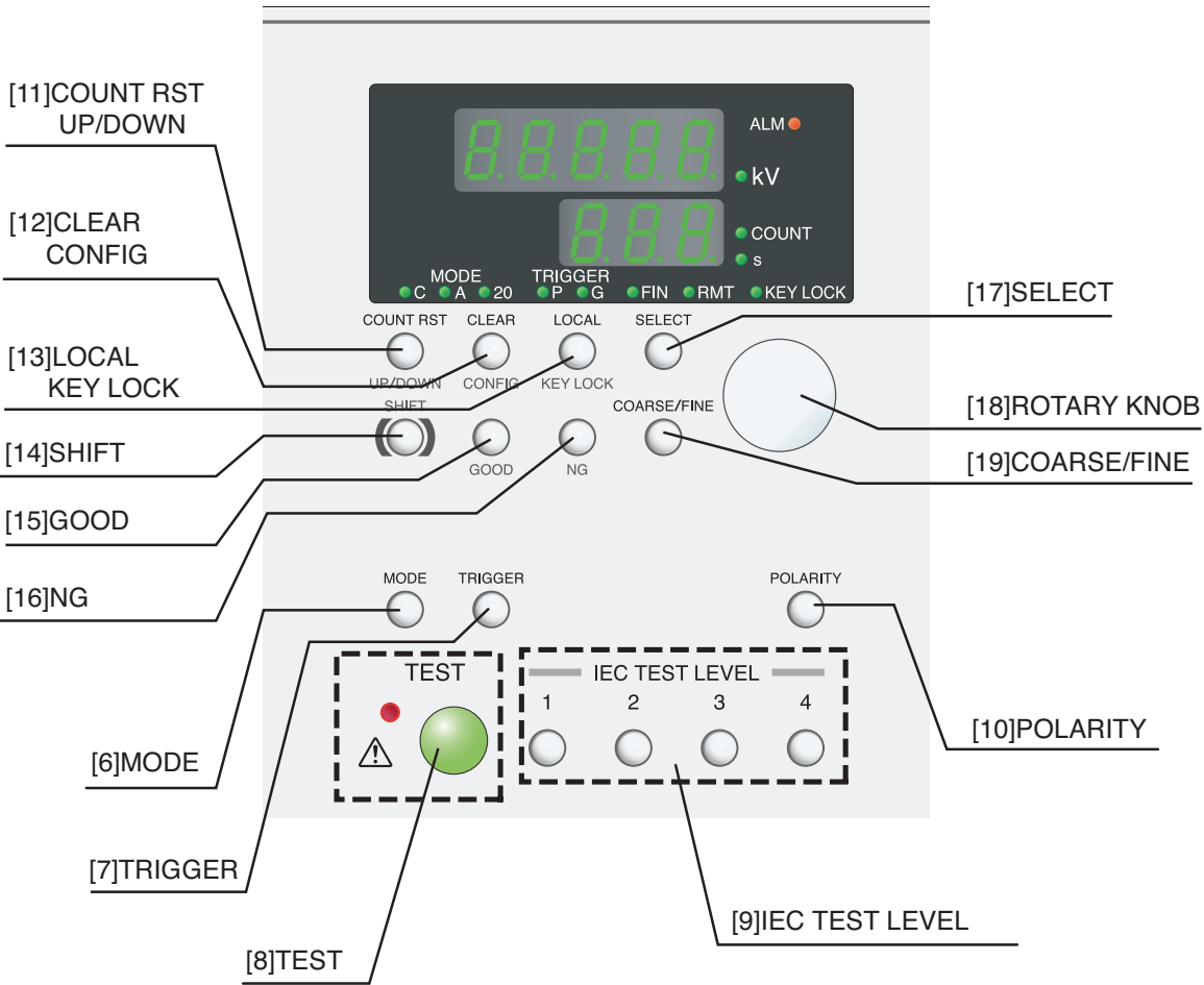
Fig. 4-2 Front Panel (Enlarged Control Section)
