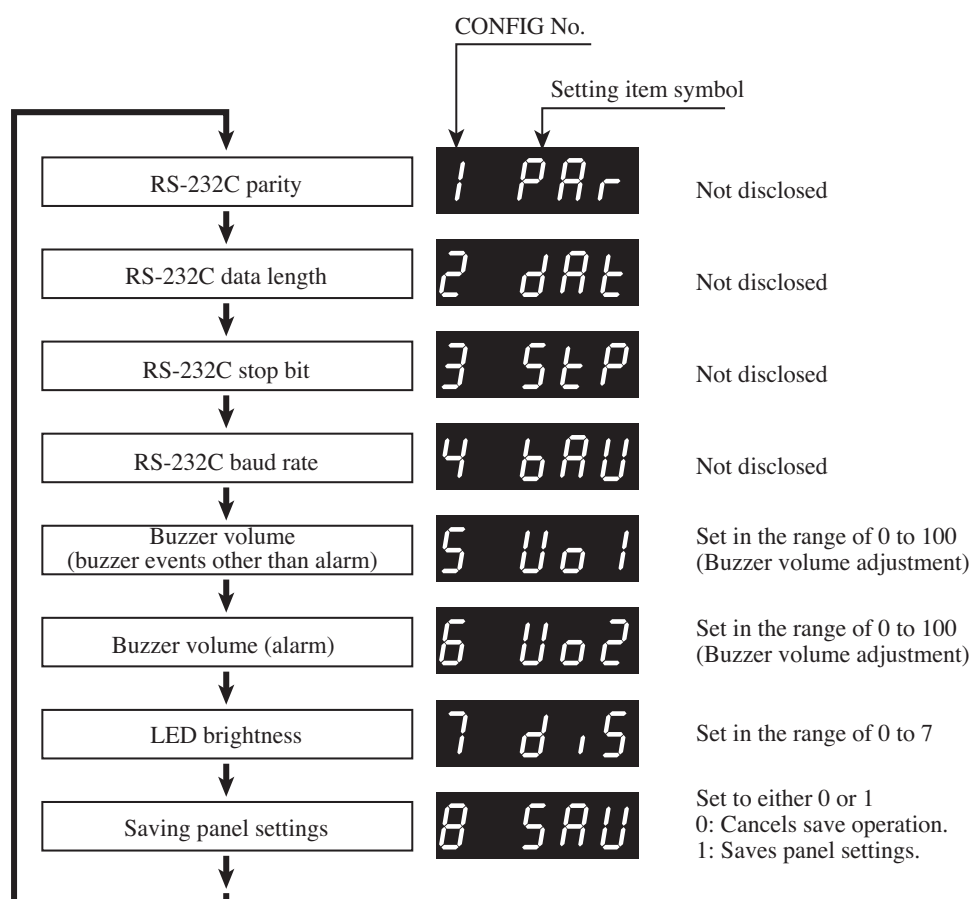
Fig. 5-3 CONFIG Setup
