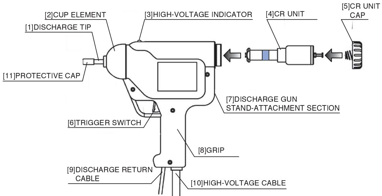
Fig. 4-5 Discharge Gun
