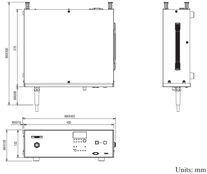
Fig. 8-2 Outline Drawing of Main Unit
